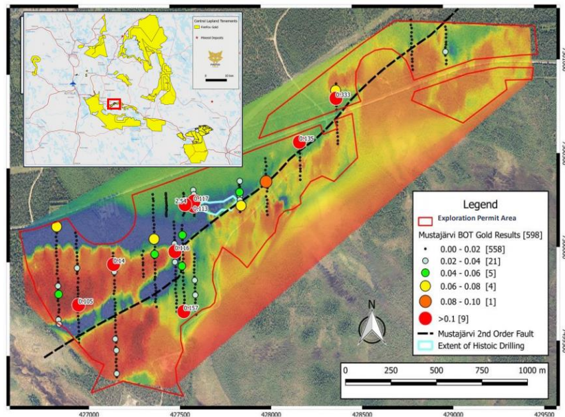
Figure 10: Mustajärvi and Central Lapland Tenements
