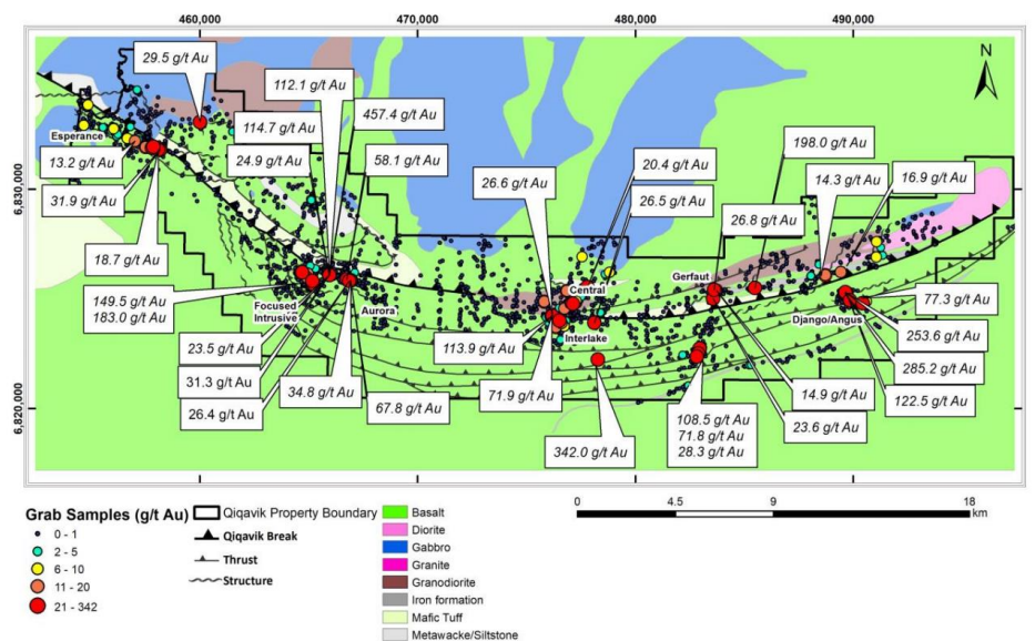
Figure 14: Qiqavik High-Grade Grab Samples
