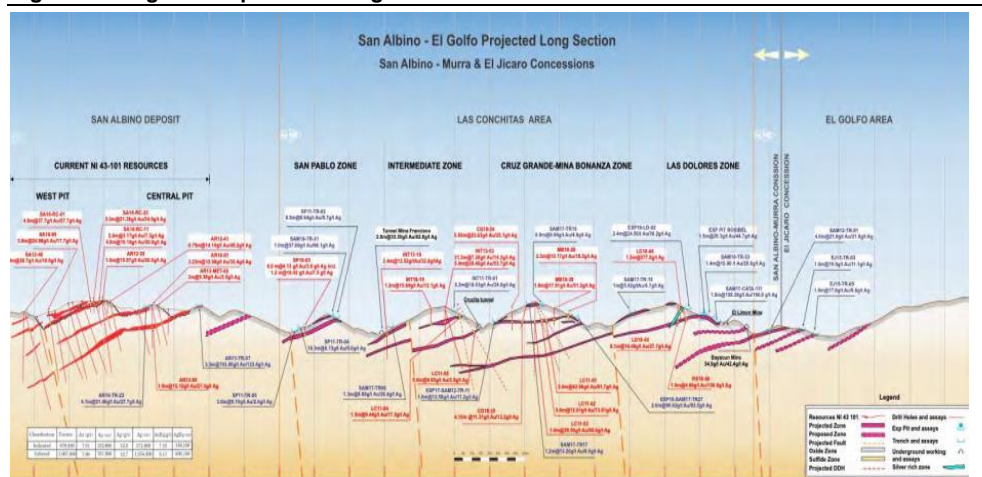
Figure 11: Regional Exploration Targets
