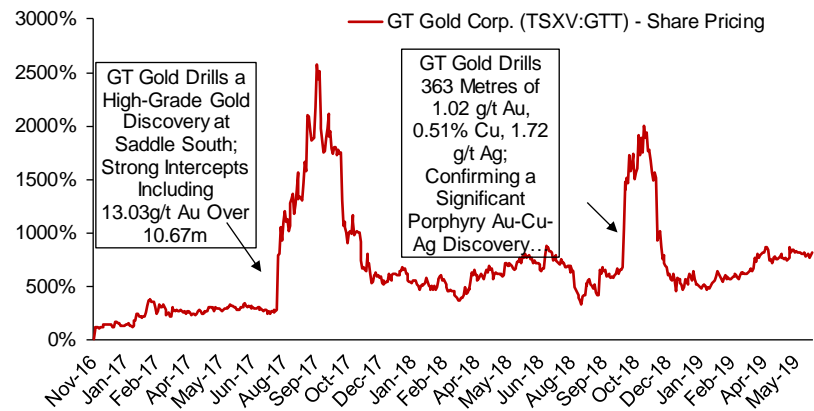
Figure 4: GT Gold – Multiple Discoveries Creates Multiple Share Price Runs
