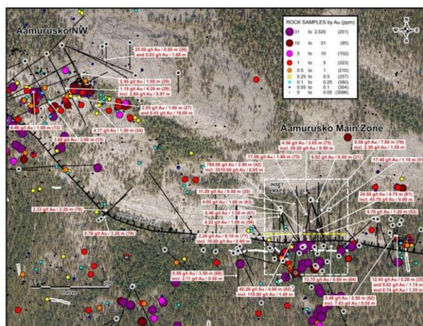
Figure 6: Drill Plan at Aamursko
