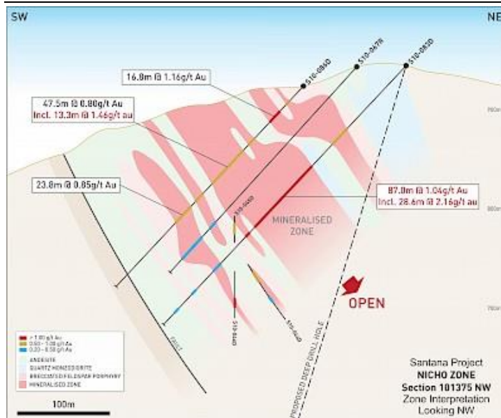
Figure 13: Cross Section Depicting Results in the Nicho Zone
