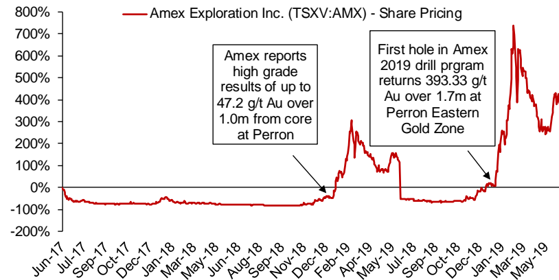
Figure 2: Amex Exploration – High-Grade Results, with Follow-up
