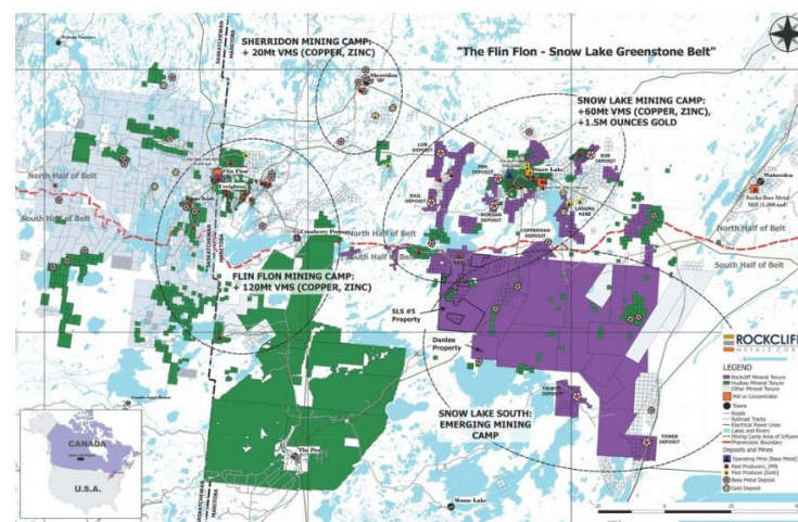
Figure 20: Rockcliff’s Prolific Base Metal Exploration Camp
