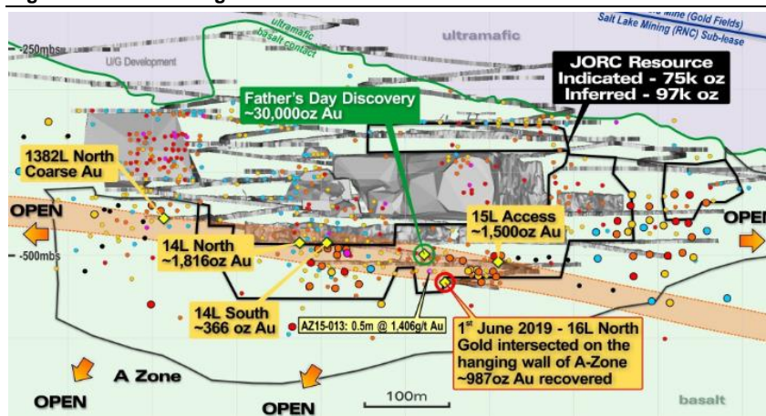
Figure 16: A Zone Long Section
