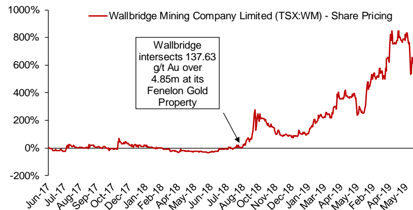
Figure 3: Wallbridge Mining – Repeating High-Grade Success
