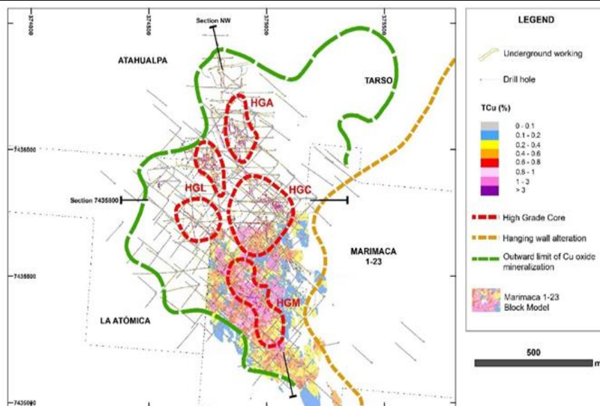
Figure 19: Copper Oxide Mineralization Mapped at Surface, Marimaca Project Property
