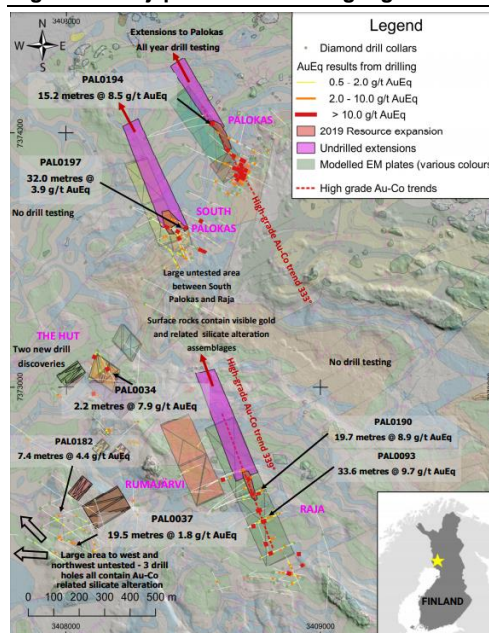
Figure 12: Rajapalot 2019 Drill Highlights
