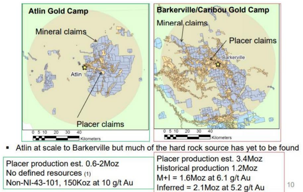
Figure 7: Atlin Comparison to Barkerville
