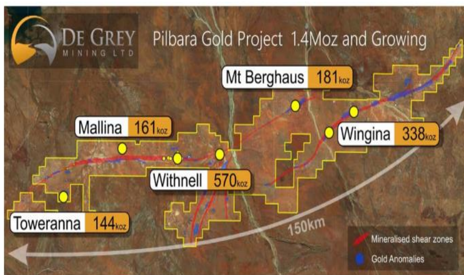
Figure 9: Pilbara Gold Project – Gold Deposits and Resources
