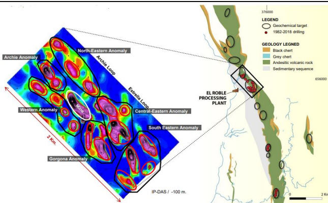
Figure 18: Regional Potential at El Roble
